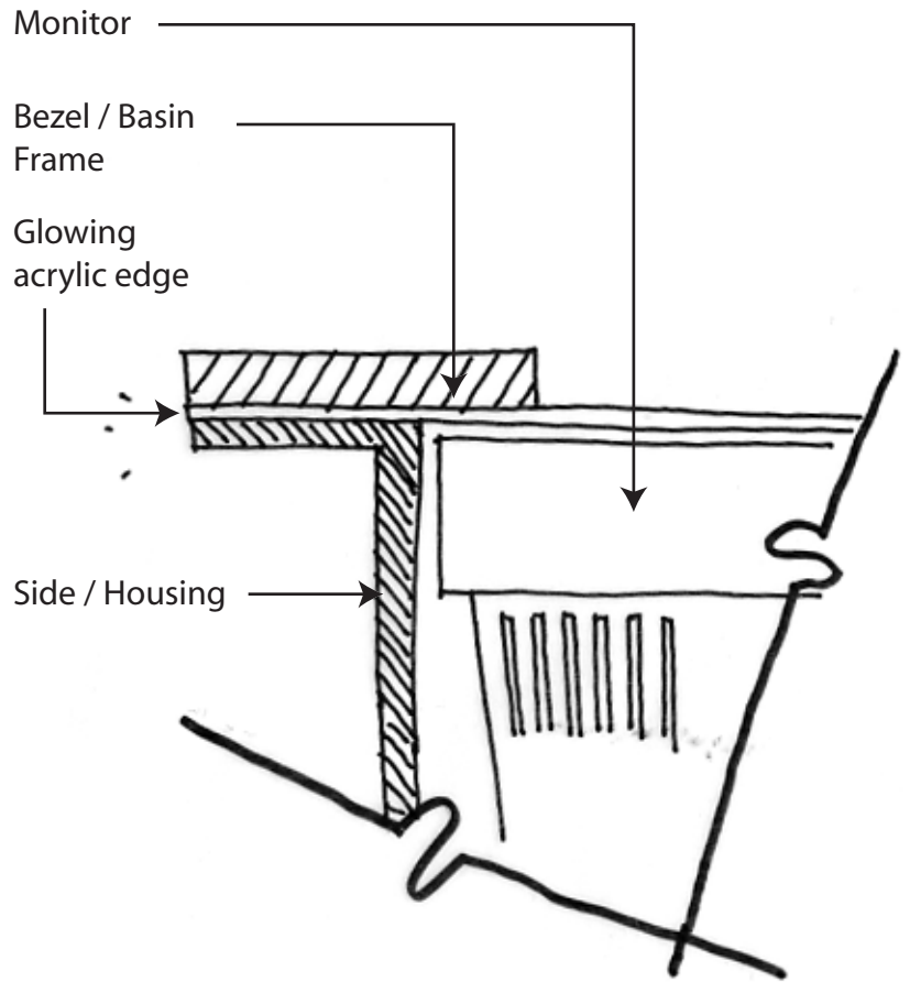
Section View Computer sits in base while monitor faces up to provide 'basin' for virtual water
